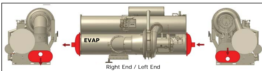
Figure 36. One-pass or three-pass non-marine (250E only)
