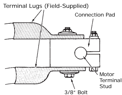
Figure 23. Electric connections
