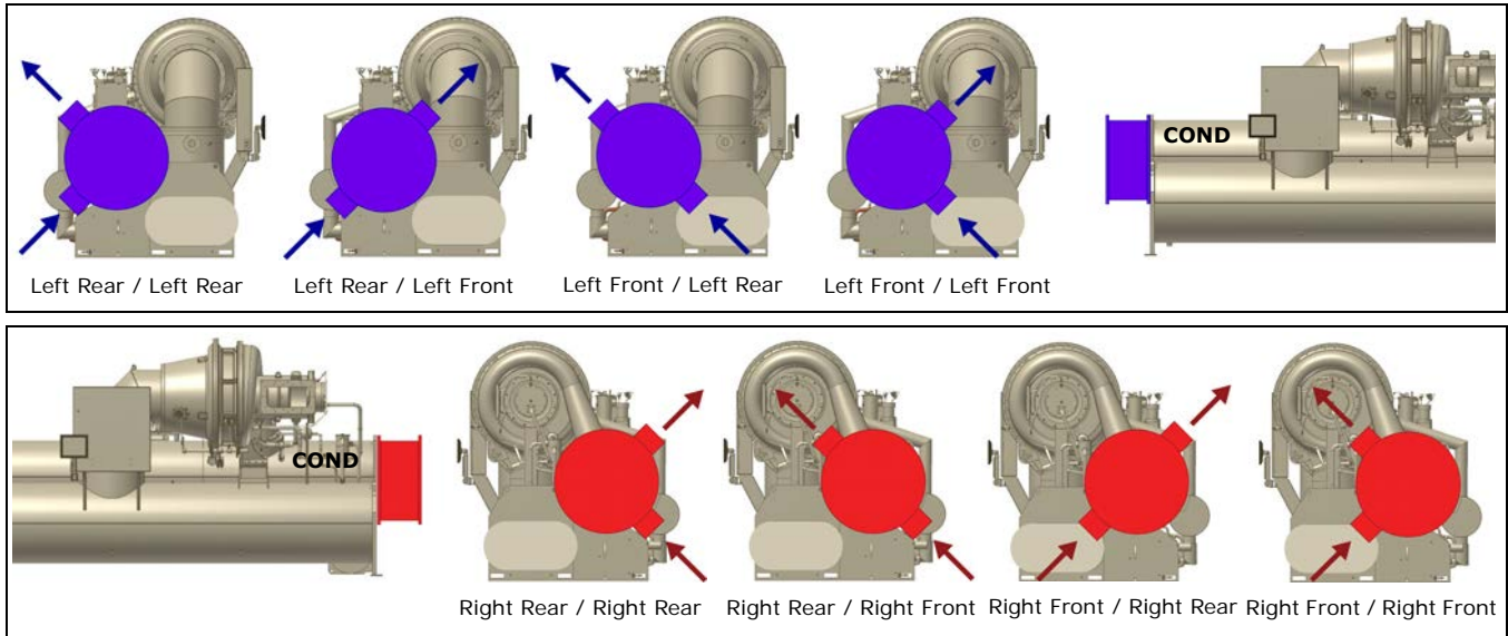
Figure 41. Two-pass marine
