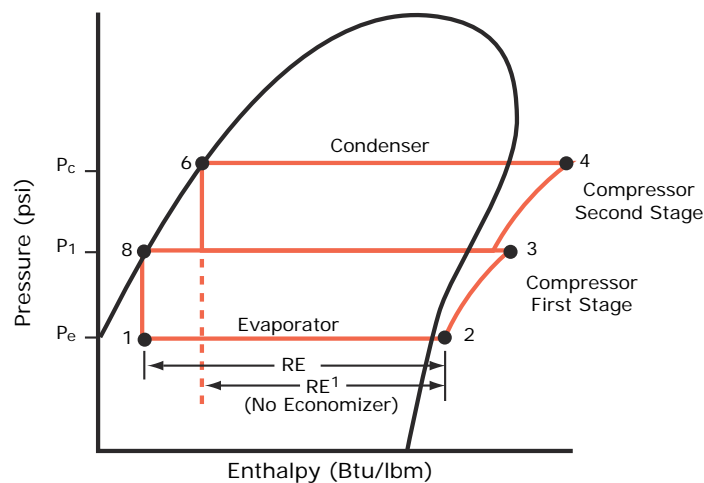
Figure 4. Two-stage CentraVac P-H diagram
