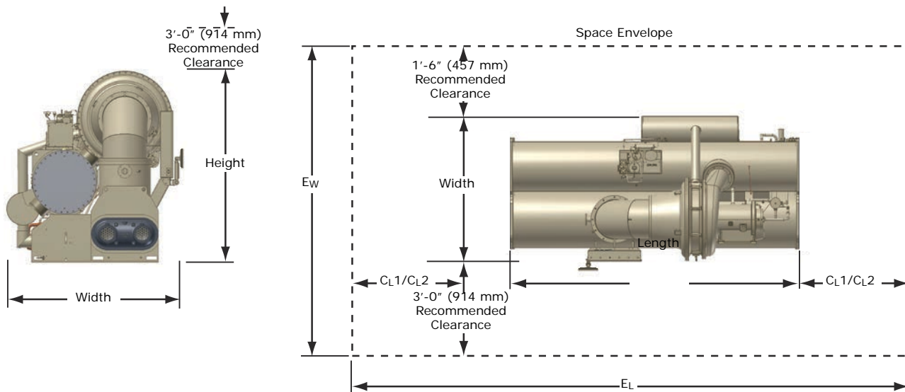
Figure 30. For Table 8, p. 71 and Table 7, p. 70: Space envelope for 50 and 60 Hz compressor chillers (a)
