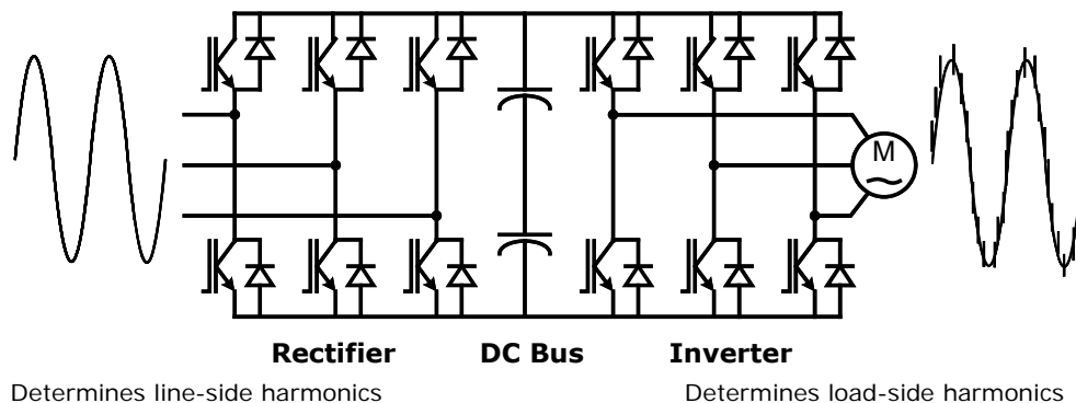
Figure 9. AFD power sections
