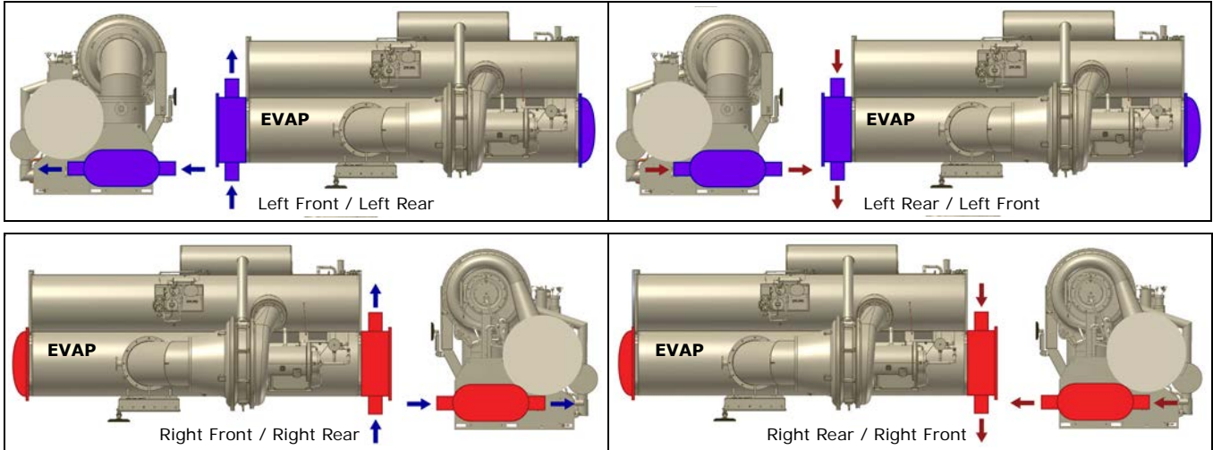
Figure 37. Two-pass marine
