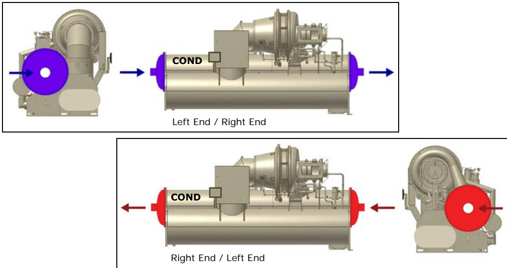
Figure 40. One-pass non-marine
