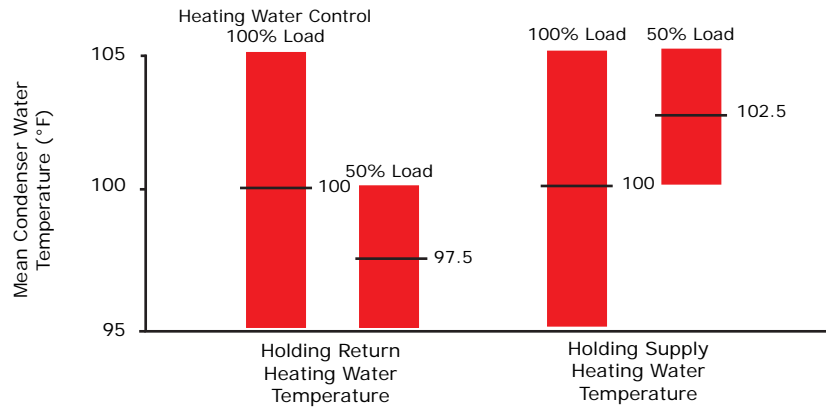
Figure 19. Heating water control
